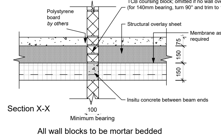
JF121 - Staggered Bearing Loadbearing Wall
