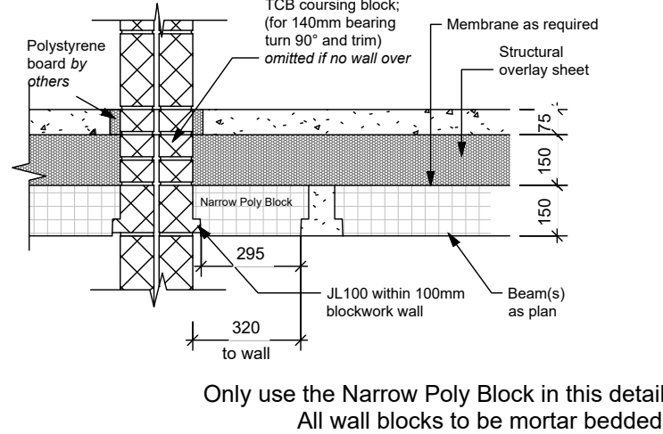
JF116 - Transverse Span, Loadbearing Wall
