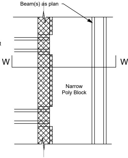
JF116 - Transverse Span, Loadbearing Wall
