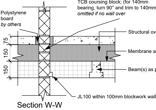
JF116 - Transverse Span, Loadbearing Wall
